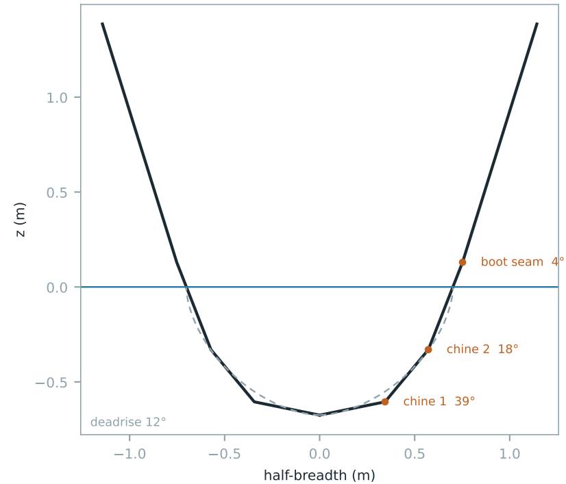
Midship section, station 6 ( x = 9.0 m) dashed: the equal-area round-bilge sibling
