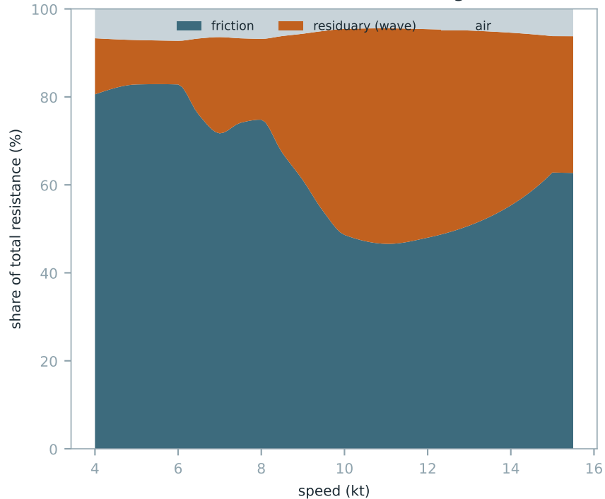
Where the drag goes friction dominates the cruise; wave-making takes over above 9 kt
