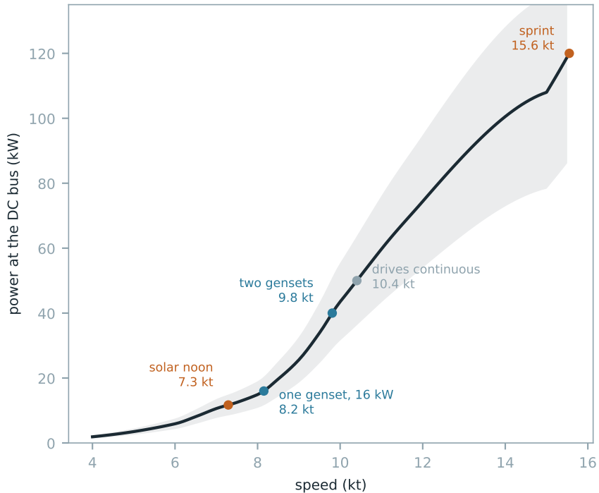
Power curve, half load shaded band is the \pm 27.5\% model uncertainty on absolutes
