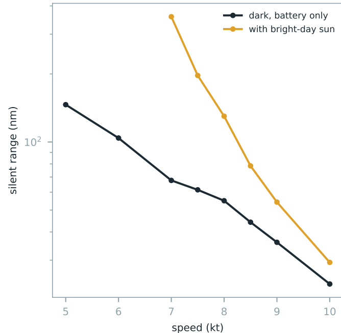
Silent range on 102 kWh usable log scale; below 7 kt the sun simply wins
