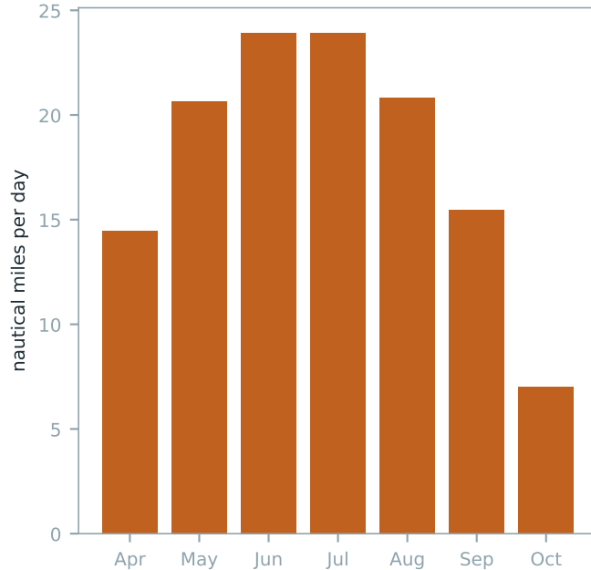
Free miles from the surplus priced at 8 kt including a 25 % weather margin
