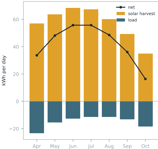
Maine season energy balance 44 deg N, 15 kWp flat-mounted
